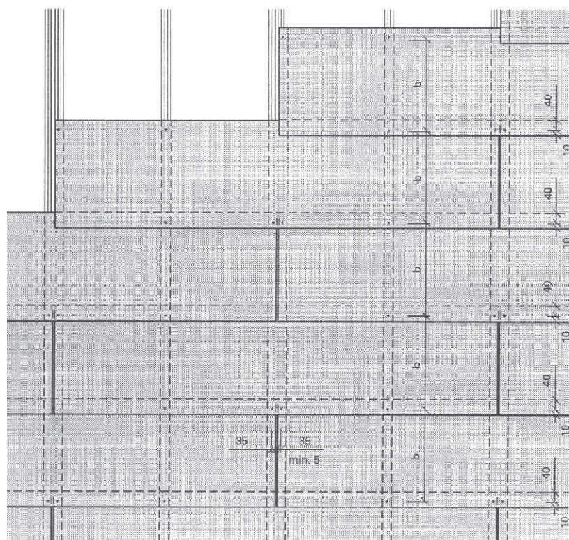
Scheme of laying of Bison Plank for Facade Sidings
